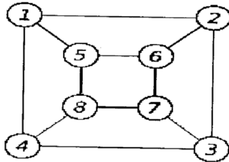
Graph G
