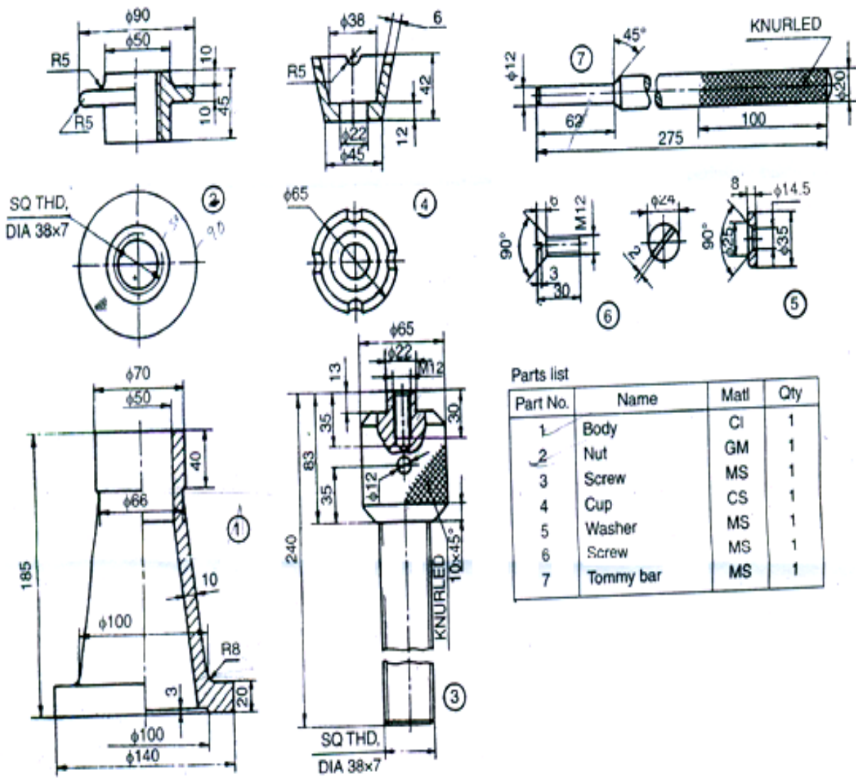
Fig. Screw jack
